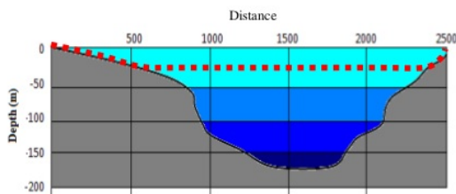
Figure-3. Suspended system pipeline installation plan.
