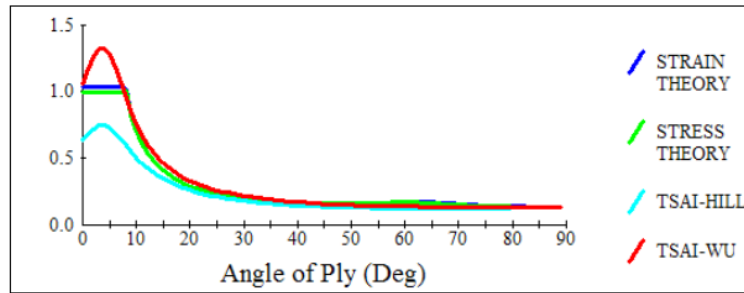
Figure 1. Strength Ratio (SR) of RFRECM
