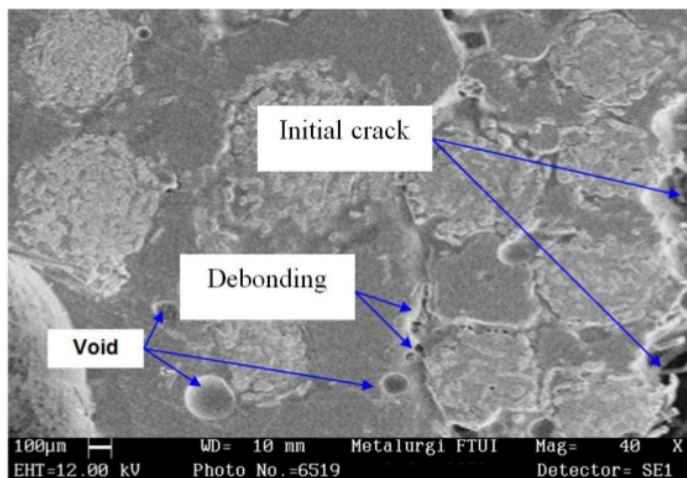
Figure 5. Morphological analysis of RFRECM by SEM
