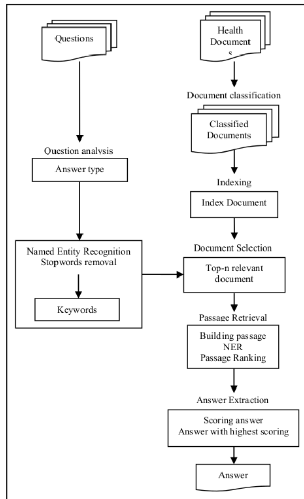
Figure 1. QA systems for Indonesian health document.
