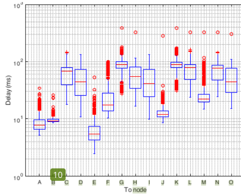
Figure 9. Sixteen-node network delay. Delay request is sent every two seconds. 1230 measurements are collected.
