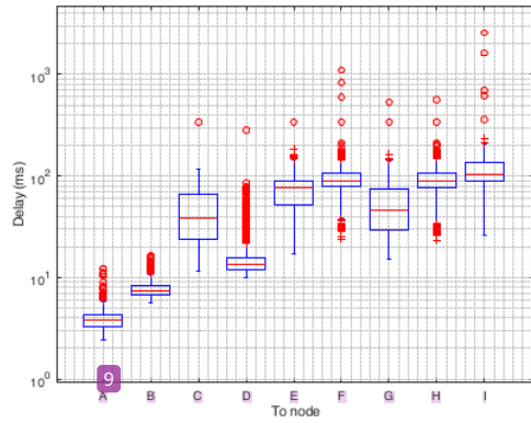
Figure 8. Ten-node network delay. Delay request is sent every two seconds. 1400 measurements are collected.
