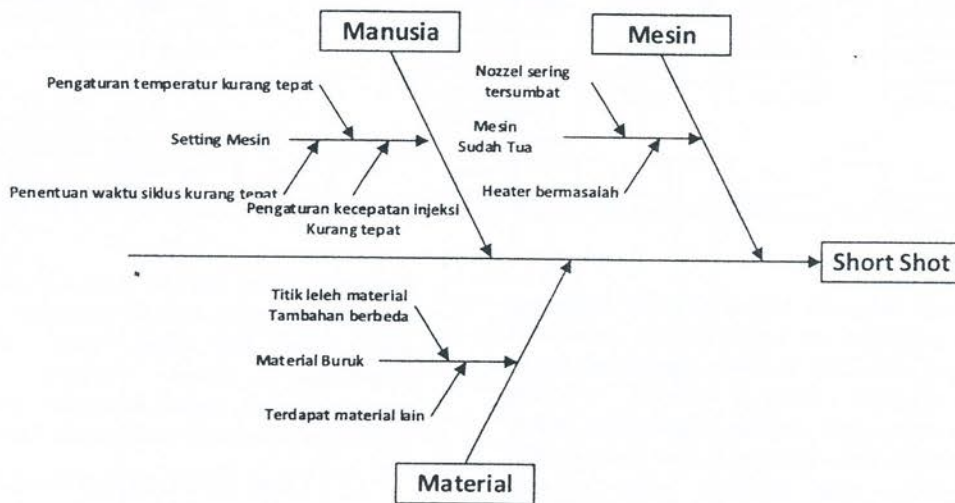
Gambar 6 Diagram Sebab Akibat Jenis Cacat Short Shot
