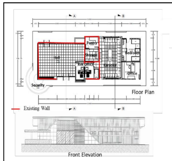
Fig. 2 Floor plan and front elevation of RW 015 office building
