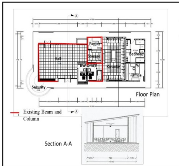
Fig. 3 Floor plan and section of RW 015 office building Source: Trisno, et al., 2019 [7]
