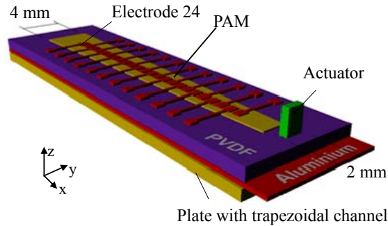
Figure 1. Schematic and dimension of PAM
