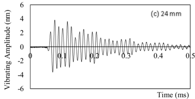
Fig. 4 Vibrating amplitude of 15 kHz at x = (a) 5, (b) 11, and (c) 24 mm
