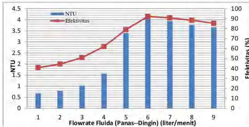
Gambar 3. Efectiveness and NTU
