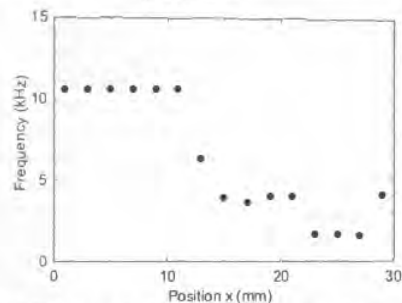
Fig.4 Relationship between position x and resonant frequency.
