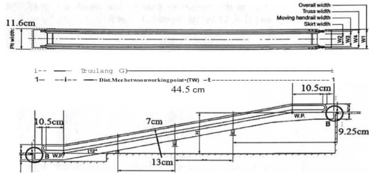
Figure 5. Escalator model design
