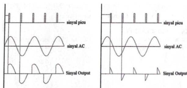
Figure 6. Large timer value (left) and small timer value (right) [3].
