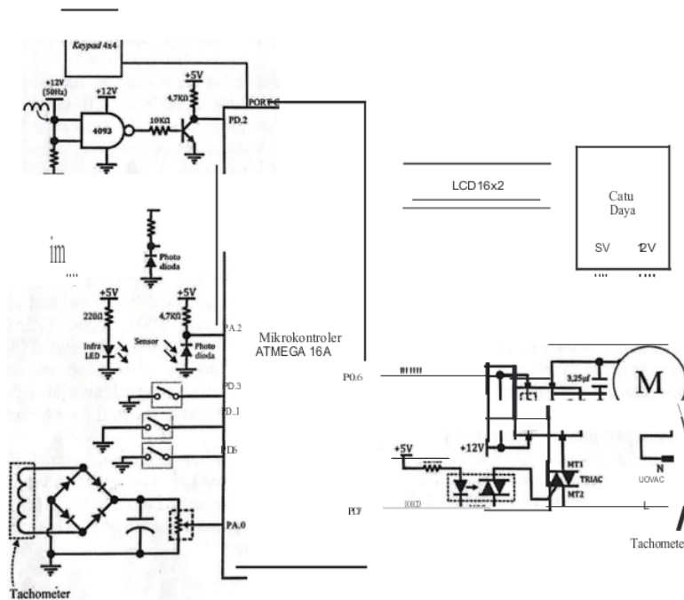
Figure 8. Complete system
