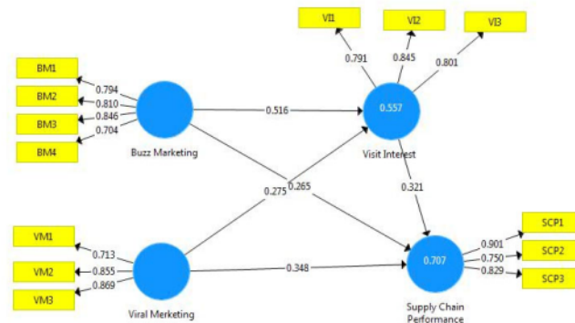
Fig. 1. Validity Testing
