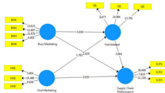
Fig. 2. Hypotheses Testing
