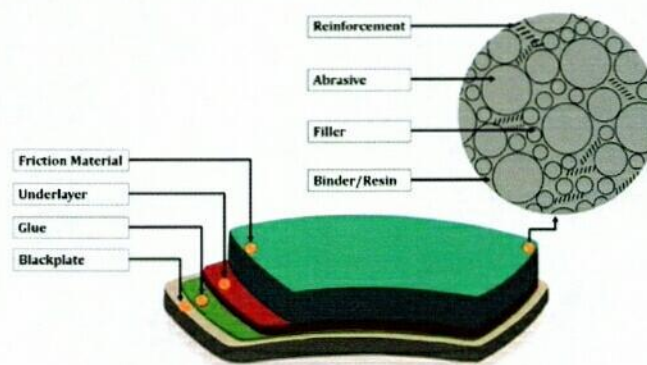
Figure 3. The layers of the brake pad.
