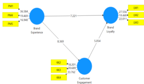
Figure 1 Bootstrapping Test Results
