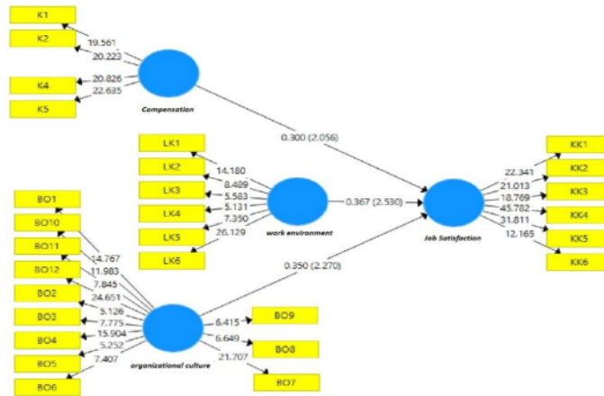
Figure 2. Bootstrapping Result
