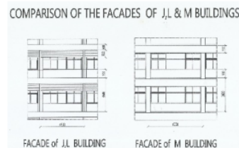
Figure 8. Vital elements of the North-South side facade in columns, parapets, windows and elongated listplank
