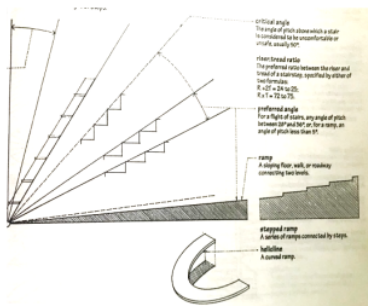
Figure 13 Preferred Angle Stair
