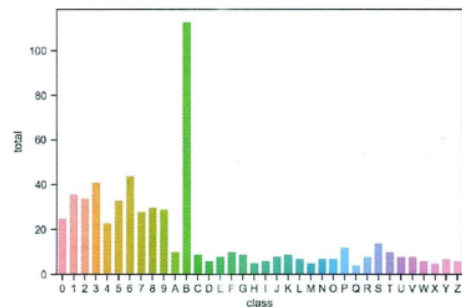
(b) Validation
