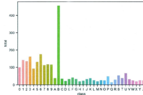
(a) Training
