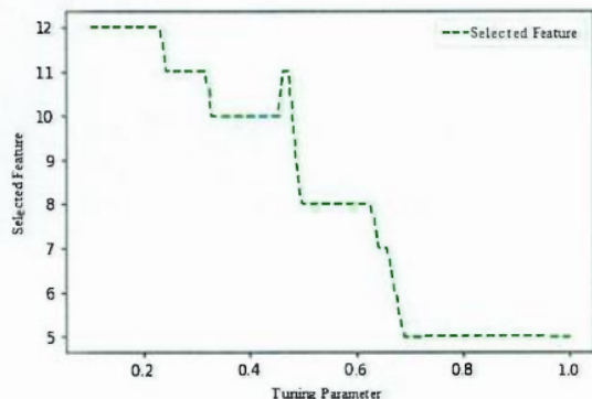
Fig. 3. Number of Selected Feature Graph
