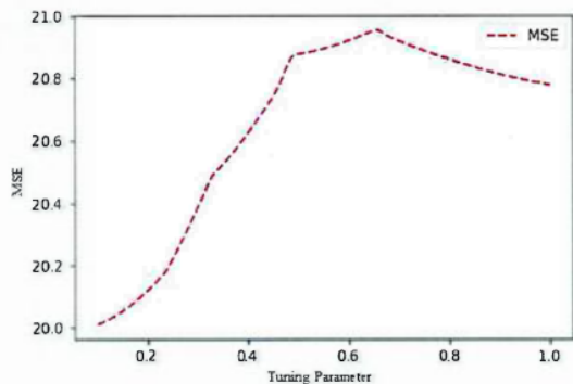
Fig. 2. MSE Graph
