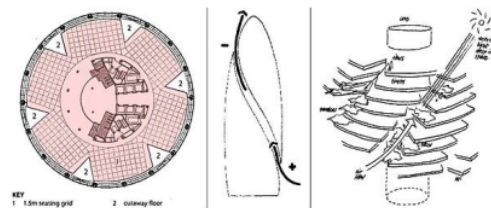
Figure 7 Air movement through the Cutaway Floor [9]
