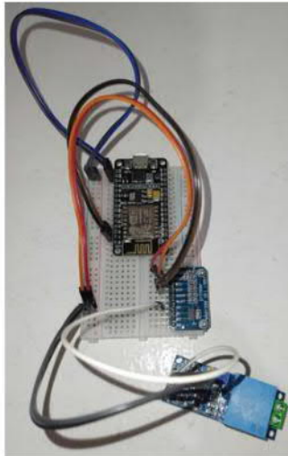
FIGURE 2. Implementation of ADS1115 to ESP8266
