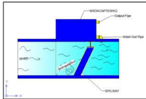
Figure 1. Top View of Intake Filtration
