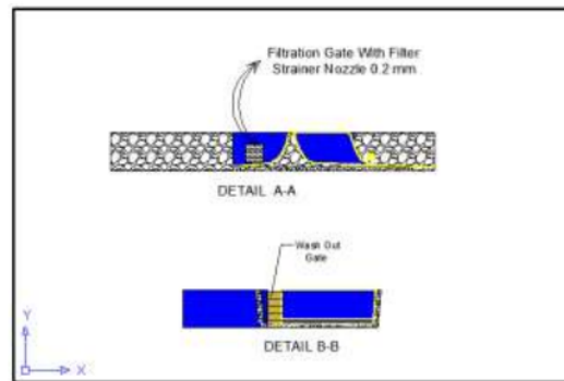
Figure 2. Side View of Intake Filtration
