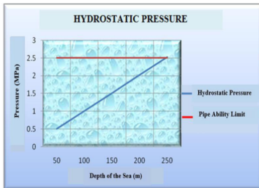
Figure-7. Pressure hydrostatic.
