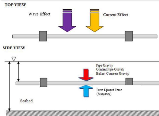
Figure-1. Forces on suspended pipe [1].
