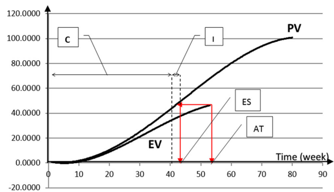
Figure 3. The concept of Earned Schedule (Source: Anondho 2018).
